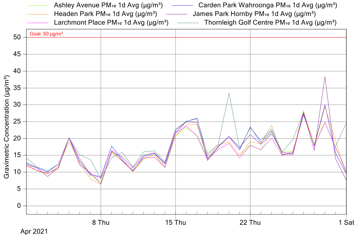
Figure 4: NorthConnex Project Air Monitoring Stations - PM 10 1 Day Averages for April 2021
