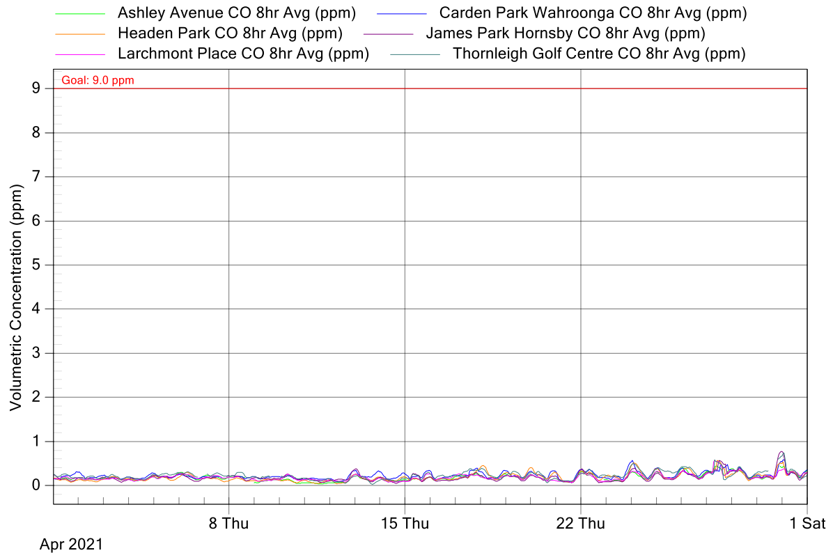
Figure 2: NorthConnex Project Air Monitoring Stations - CO 8 Hour Rolling Averages for April 2021
