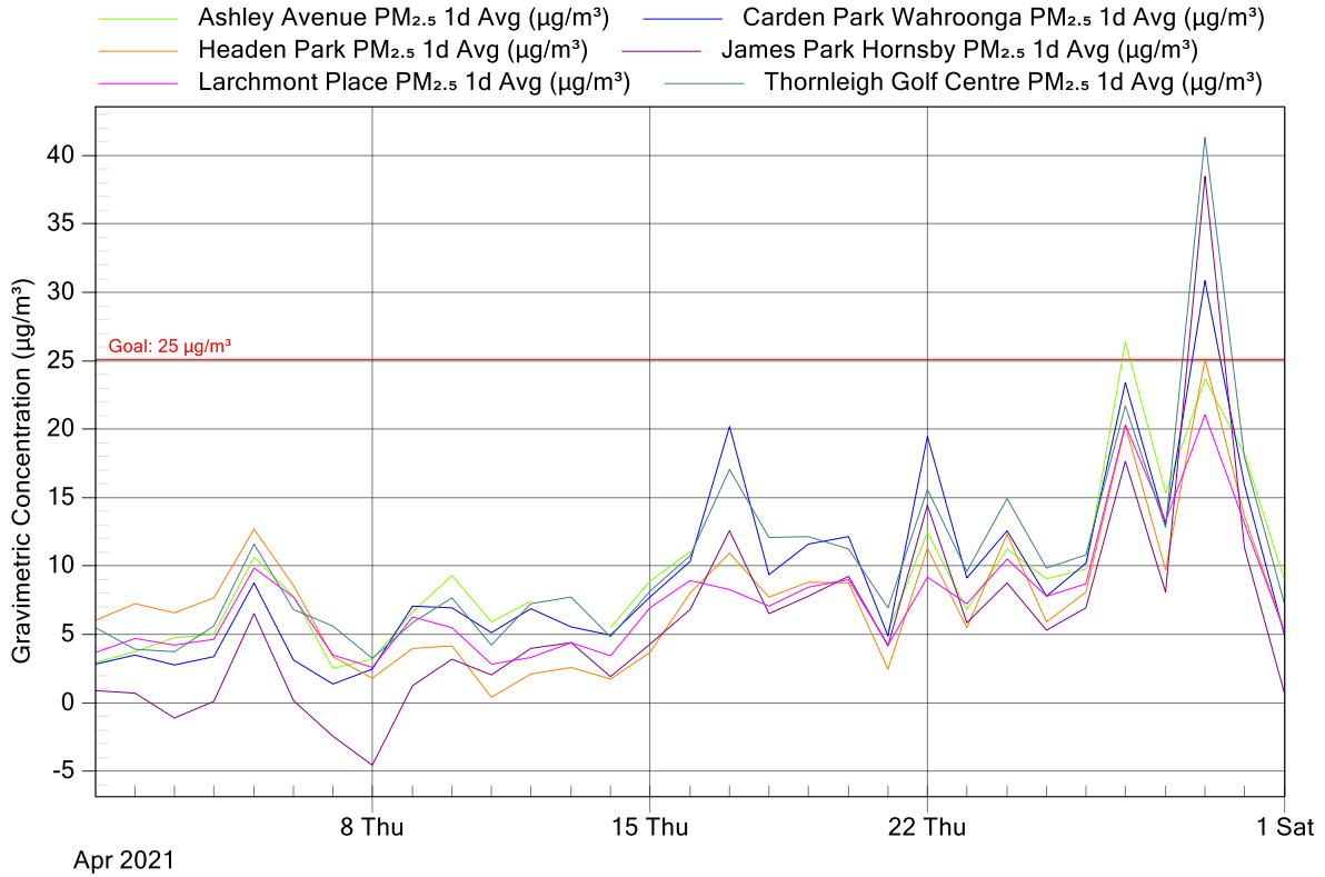
Figure 5: NorthConnex Project Air Monitoring Stations - PM 2.5 1 Day Averages for April 2021
